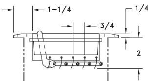
VM END VIEW
