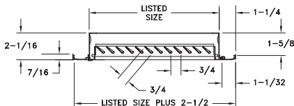
RHF45 SIDE VIEW
